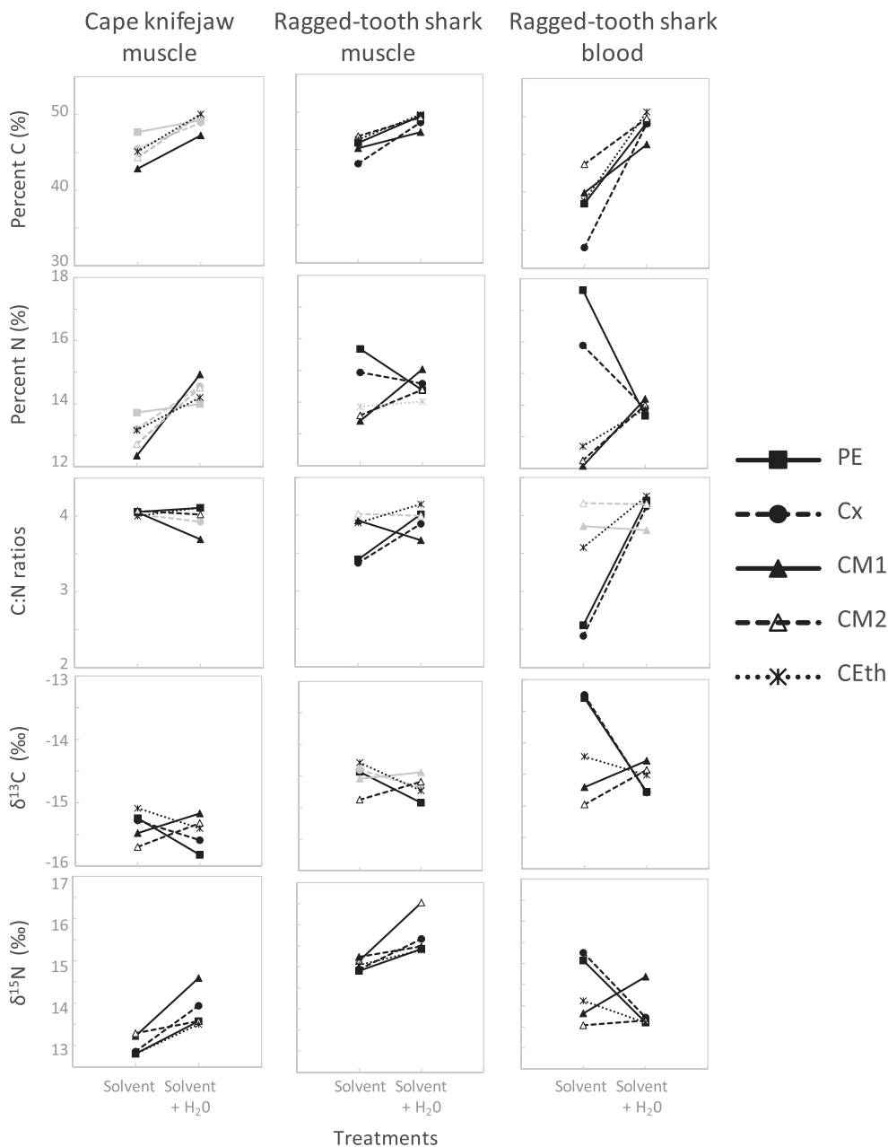
FIGURE 3 Effect of subsequent water wash after initial solvent wash on carbon percentage, nitrogen percentage, C:N atomic ratios, and \delta^{13}\text{C} and \delta^{15}\text{N} values. Significant changes are in black. (Refer to Figure 1 for abbreviations)
