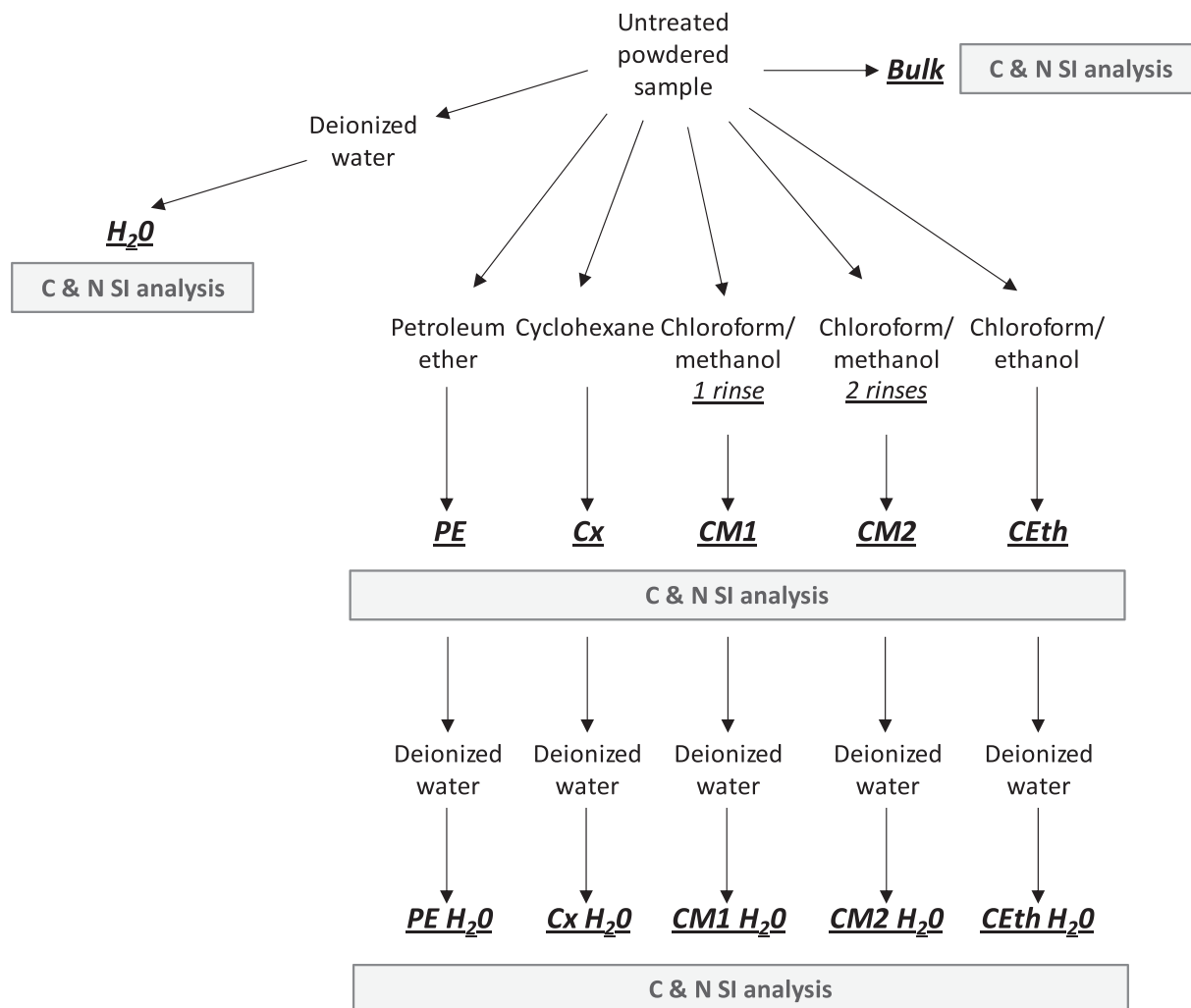
FIGURE 1 Schematic representation of the various pre-treatments tested. SI: stable isotope
