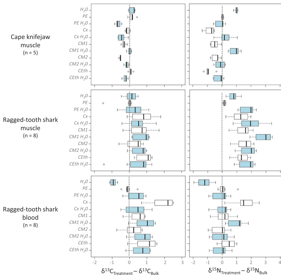
FIGURE 4 Changes in \delta^{13}\text{C} and \delta^{15}\text{N} values after the eleven pre-treatments relative to the untreated bulk samples of the three tissues (Cape knifejaw muscle, ragged-tooth shark muscle and blood). The data for water-rinsed tissues are in blue. (Refer to Figure 1 for abbreviations) [Color figure can be viewed at wileyonlinelibrary.com ]
