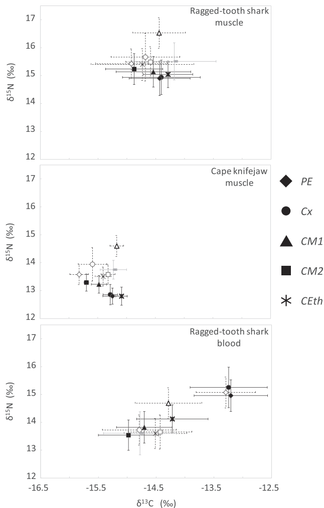
FIGURE 5 Carbon and nitrogen stable isotope ratios (mean \pm SD) of ragged-tooth shark muscle and blood and Cape knifejaw after water treatment (grey), solvent treatment (black), and solvent and water treatments (dotted line). (Refer to Figure 1 for abbreviations)
