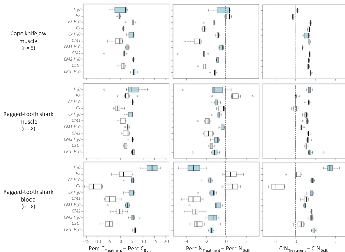
FIGURE 2 Changes in carbon and nitrogen percentages (Perc. C and Perc. N, respectively) and C:N ratios after the eleven pre-treatments relative to the untreated Bulk samples (Cape knifejaw muscle, ragged-tooth shark muscle and blood). The data for water-rinsed tissues are in blue. (Refer to Figure 1 for abbreviations) [Color figure can be viewed at wileyonlinelibrary.com ]
